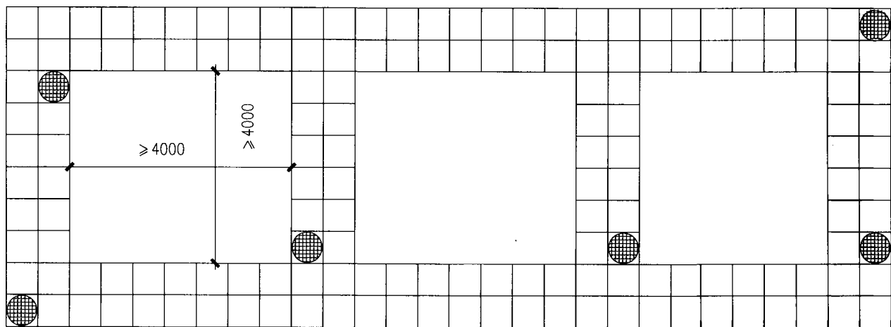
(2) 梯形布置
